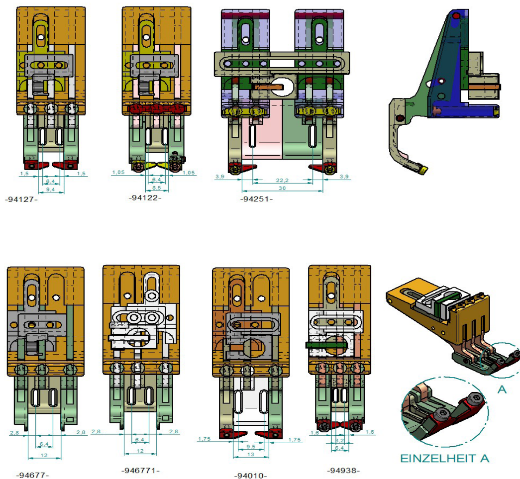
Three-part double-needle tape sewing feet
