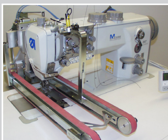
Additional transport small on a double needle lockstitch machine
