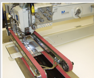
Additional transport small additional transport for straight seams mounted directly on the sewing machine
