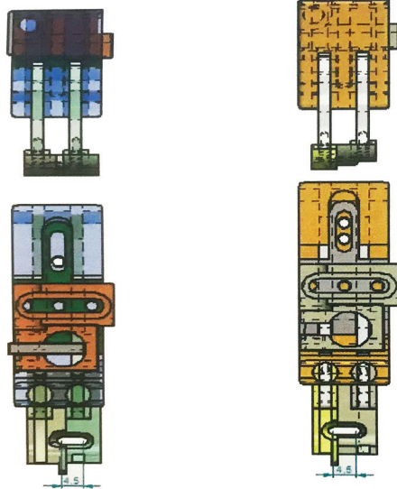
94794 Singer, Juki, Brother - 94468 Pfaff, Durkopp Haftenband, adhesive tape presser foot
