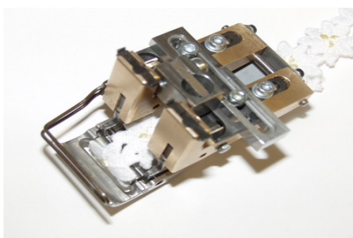
Zigzag sewing foot with an overstretch of 10 mm Art. no.: MK_94911
