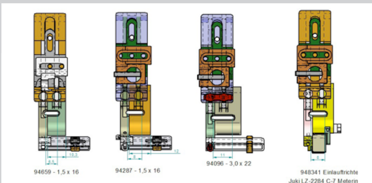
Zigzag rubber compensating sewing feet for sewing on and over rubber braid. Braid guide attached to left sole
