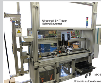
Ultrasonic welding machine for fully automatic production of bra straps with closure component
