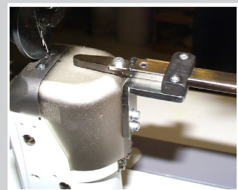
Pneumatic edge stop, small version for post bed machine
