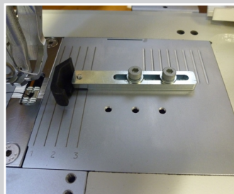
Simple edge guide on base plate for straight seams
