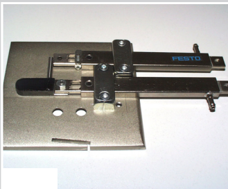
double cylinder, small version for two positions
