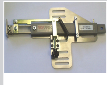
Pneumatic edge stop, with big cylinder for three positions
