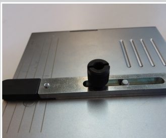
Simple edge stop on base plate for radii
