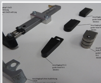
Pneumatic fabric edge stop to right of needle with cylinder for two edge distances and different stop heads
