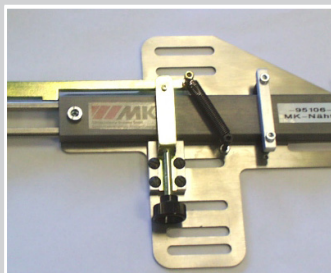
Fabric edge stop on base plate with several edge distances
