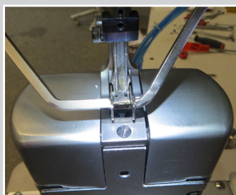
Swing-up fabric edge stop for right and left of needle
