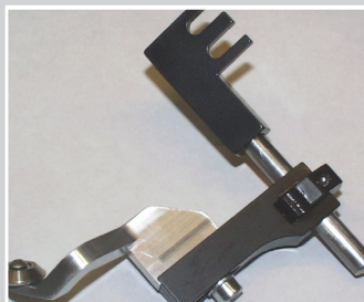
Swing-up fabric edge stop with inclined guide roller
