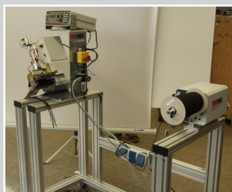
Hot wire cutting device 60 mm with tape dispenser on rollers
