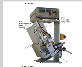
Hot wire cutting device 60 mm
