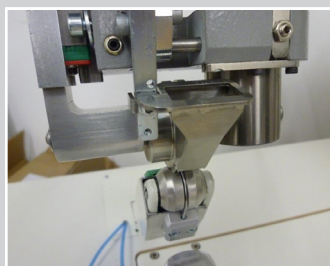
Hot air machine with height compensation roller
