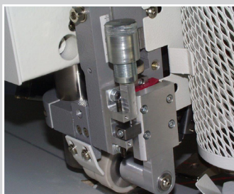
Compensatory roller from behind
