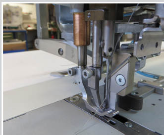
Counter knife on a flatbed/ drop feed/sewing machine, hook on left, knife stroke of 2.0 to 8.0 mm.
