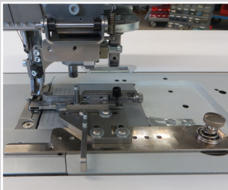
Counter knife on a flatbed/ drop feed/sewing machine, hook on right, with integrated Piping Guide
