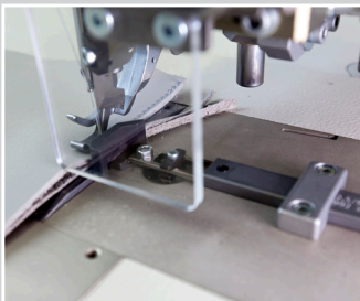
Counter knife normal version, on a flatbed/wheel feed/ sewing machine with pneumatic edge stop
