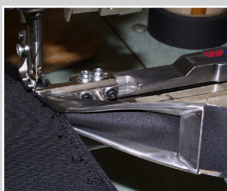
Slanted binding on a single-needle sewing machine
