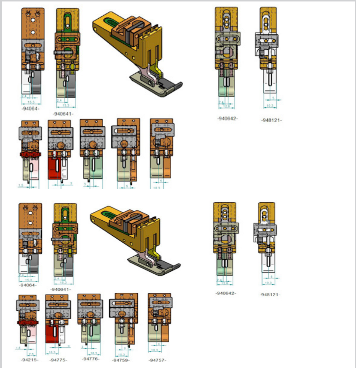
Sewing feet for one and two-part chainstitch machines
