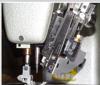
Tape feed with cutter on a lock-stitch machine
