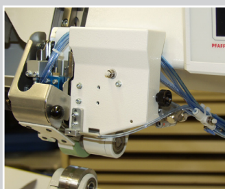
Tape feed with cutter for a hot air sealing machine with cool roller for high sealing temperatures
