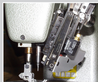
Tape feed with cutter on a lock-stitch machine
