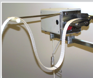
Large tape dispenser with transport roller 100 mm and dancer control
