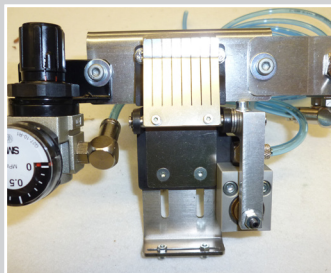
Pneumatic tape brake
